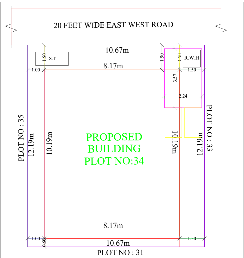
SITE PLAN NOT TO SCALE
