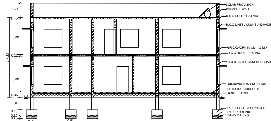
SECTION ON 'ABCD'
