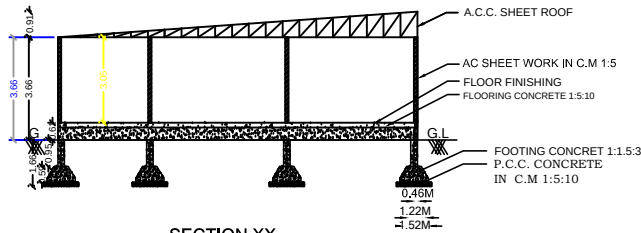
SECTION XX
