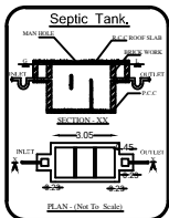
SECTION XX
