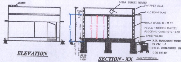
SECTION - XX
