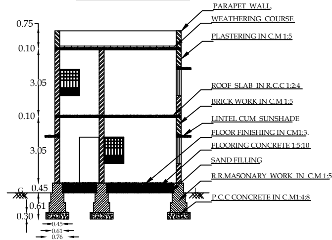
Section On-XY
