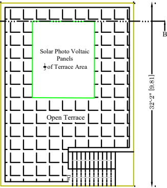
ROOF FLOOR PLAN
