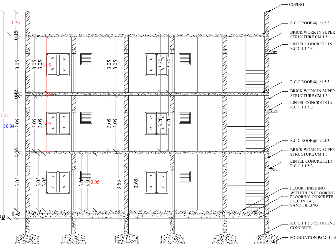
SECTION-AB
