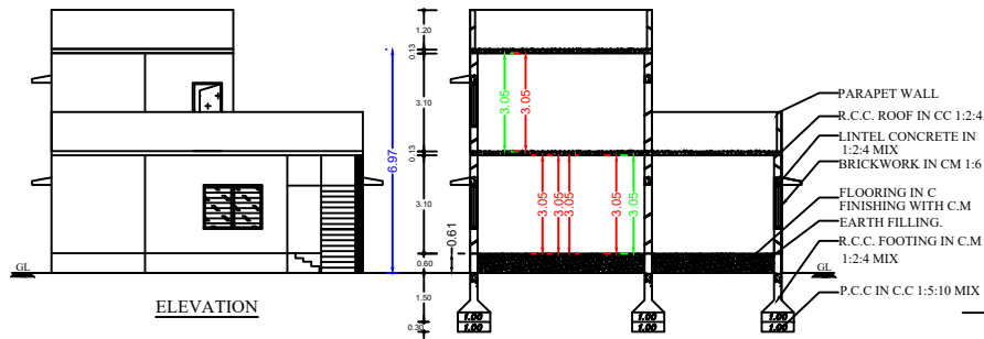
SECTION HK'
