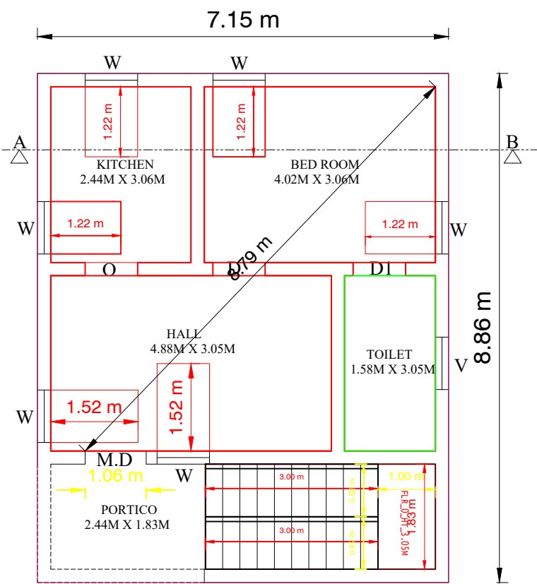
PLAN [NORTH FACING]
