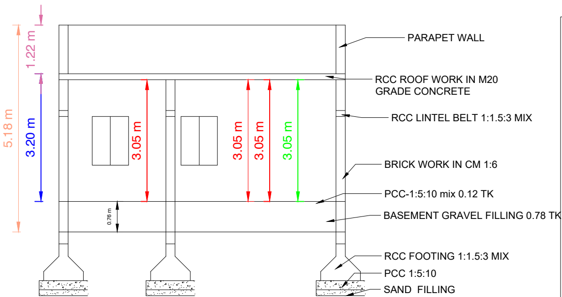
SECTION"AB"
