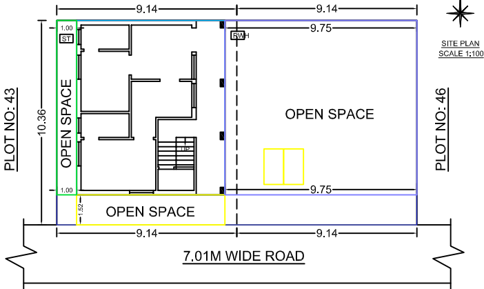
THANGAVEL PREMISES LAND
