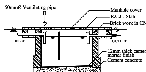
Longitudinal Section (SEPTIC TANK)
