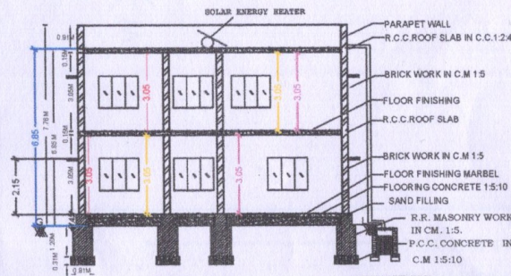
SECTION - XX
