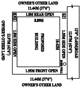
SITE PLAN
