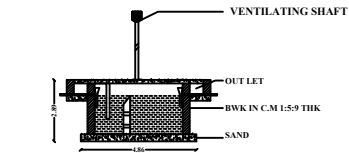
SECTION OF THE SEPTIC TANK
