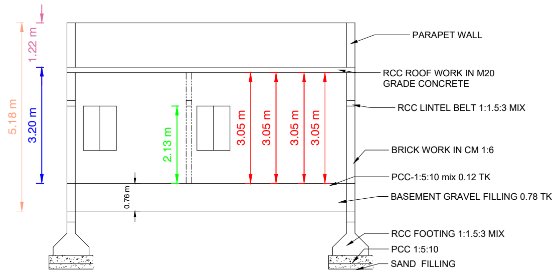
SECTION"AB"
