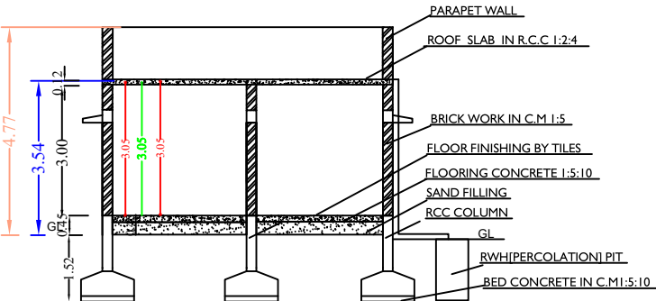
SECTION ON-XY
