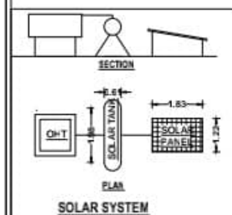
SOLAR SYSTEM
