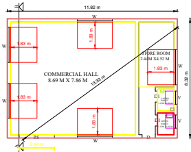
COMMERCIAL - PLAN
