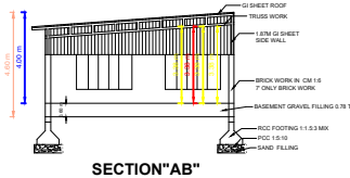
SECTION"AB"
