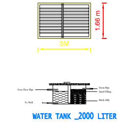
WATER TANK _2000 LITER
