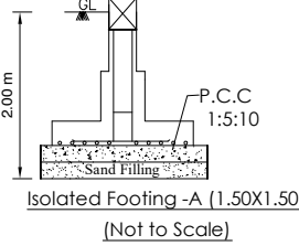
Waste Water Recycle Unit Not To Scale
