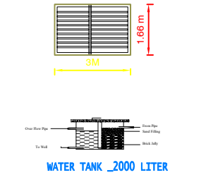
WATER TANK _2000 LITER
