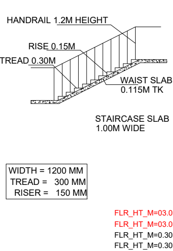
DETAILS OF STAIRCASE SCALE 1:50
