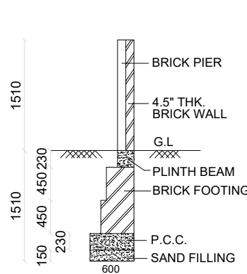
DETAILS OF COMPOUND WALL SCALE 1:50
