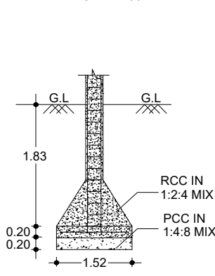
DETAILS OF RCC COLUMN SCALE 1:50
