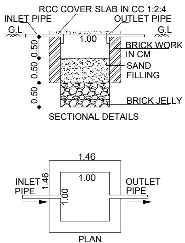
DETAILS OF ORGANIC FILTRATION BED SCALE 1:50
