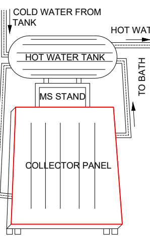
DETAILS OF SOLAR WATER HEATER SYSTEM
