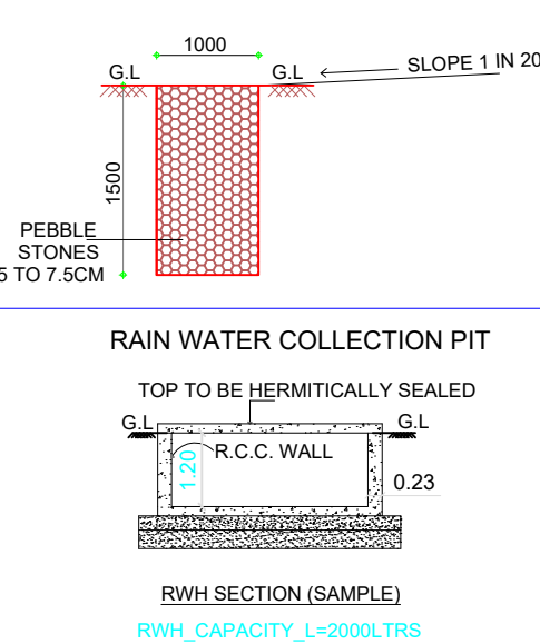
SECTION OF PEBBLE TRENCH SCALE - 1:100
