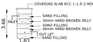
WASTE WATER RECYCLE UNIT
