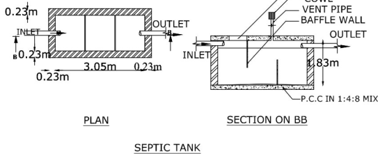
SEPTIC TANK
