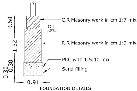
FOUNDATION DETAILS
