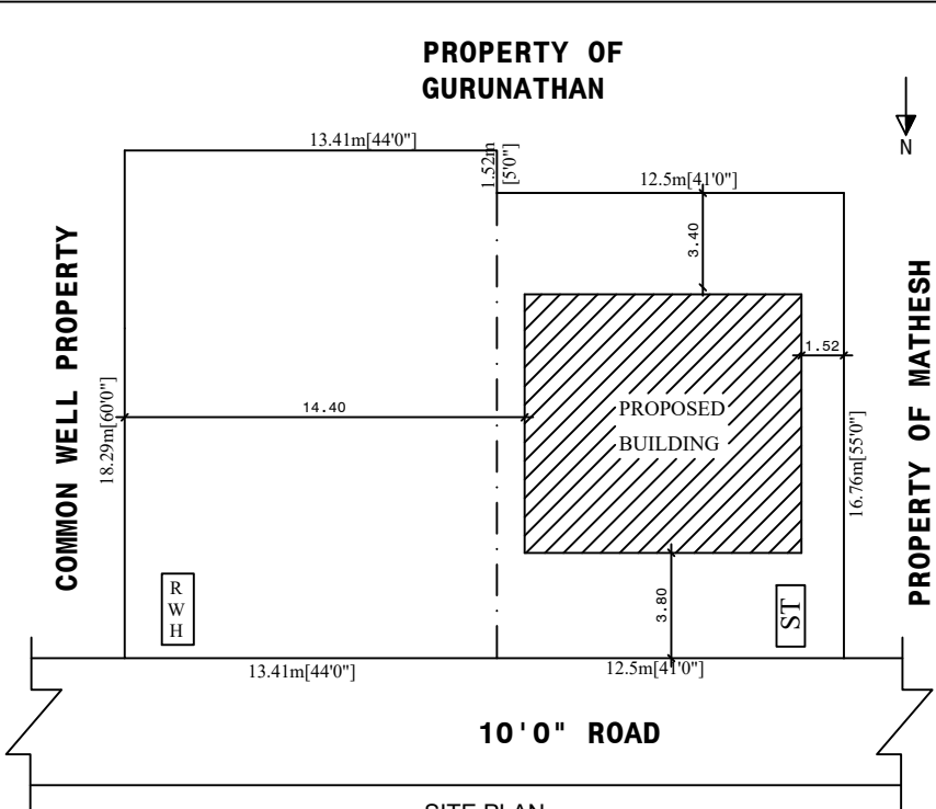
SITE PLAN SCALE:1"=8'0" [1:100]
