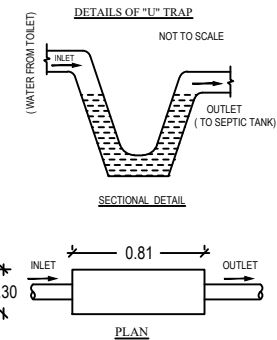
DETAILS OF "U" TRAP
