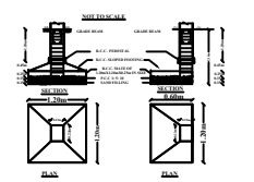
COLUMN FOOTING DETAILS
