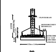
TYP.DET. COLUMN FOOTING
