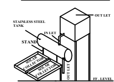
SOLAR HEATING WATER SYSTEM
