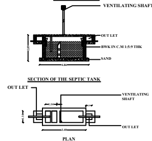
SEPTIC TANK
