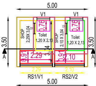
GROUND FLOOR PLAN (Scale 1:100)
