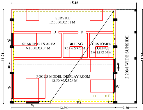
GROUND FLOOR [ SOUTH PART] - PLAN
