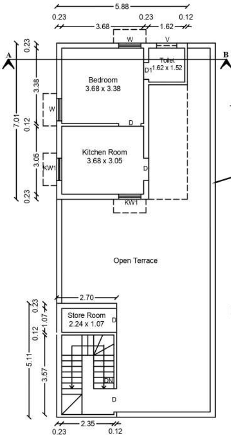
FIRST FLOOR PLAN (PROPOSED)
