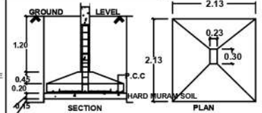
FOUNDATION DETAILS
