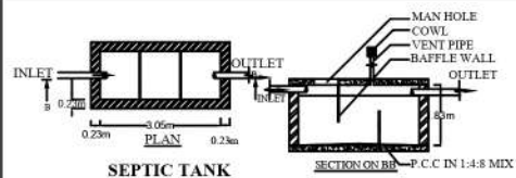
SEPTIC TANK
