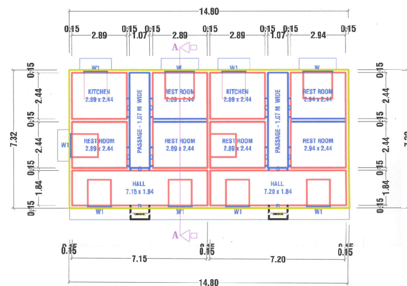
PLAN
