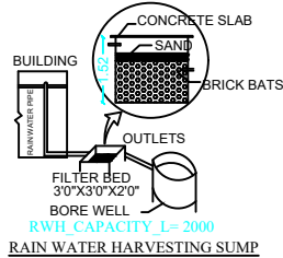
RAIN WATER HARVESTING SUMP
