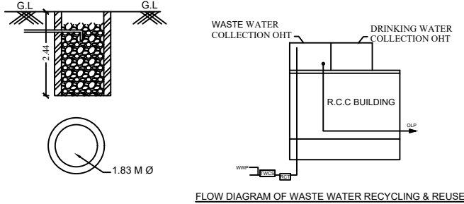
FLOW DIAGRAM OF WASTE WATER RECYCLING & REUSE
