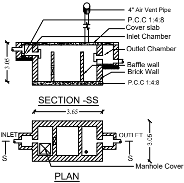
SEPTIC TANK & SOAK PIT DETAILS
