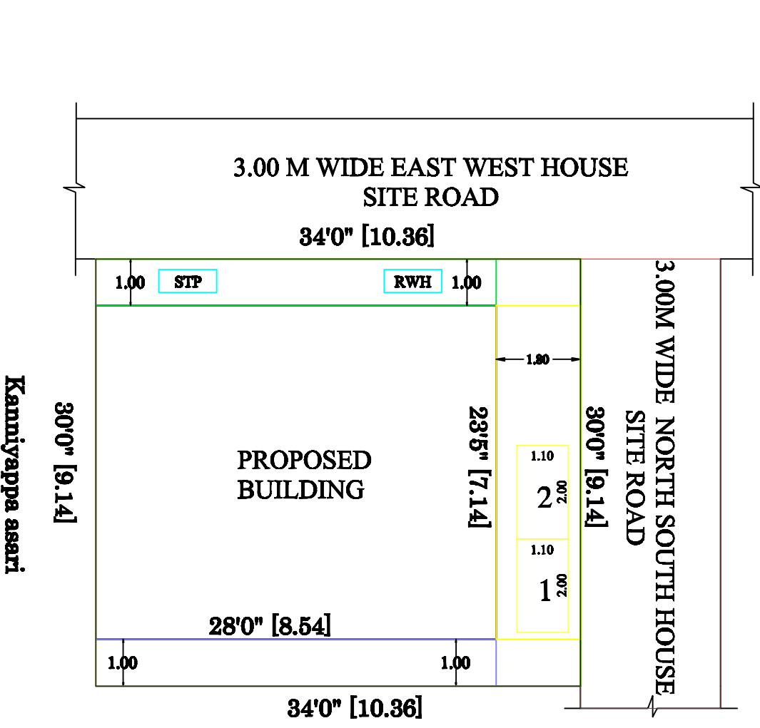
SITE PLAN
