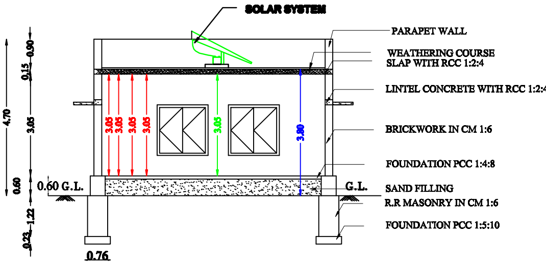
SECTION ON-'AB'
