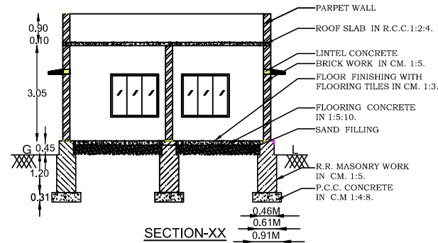
SECTION-XX
