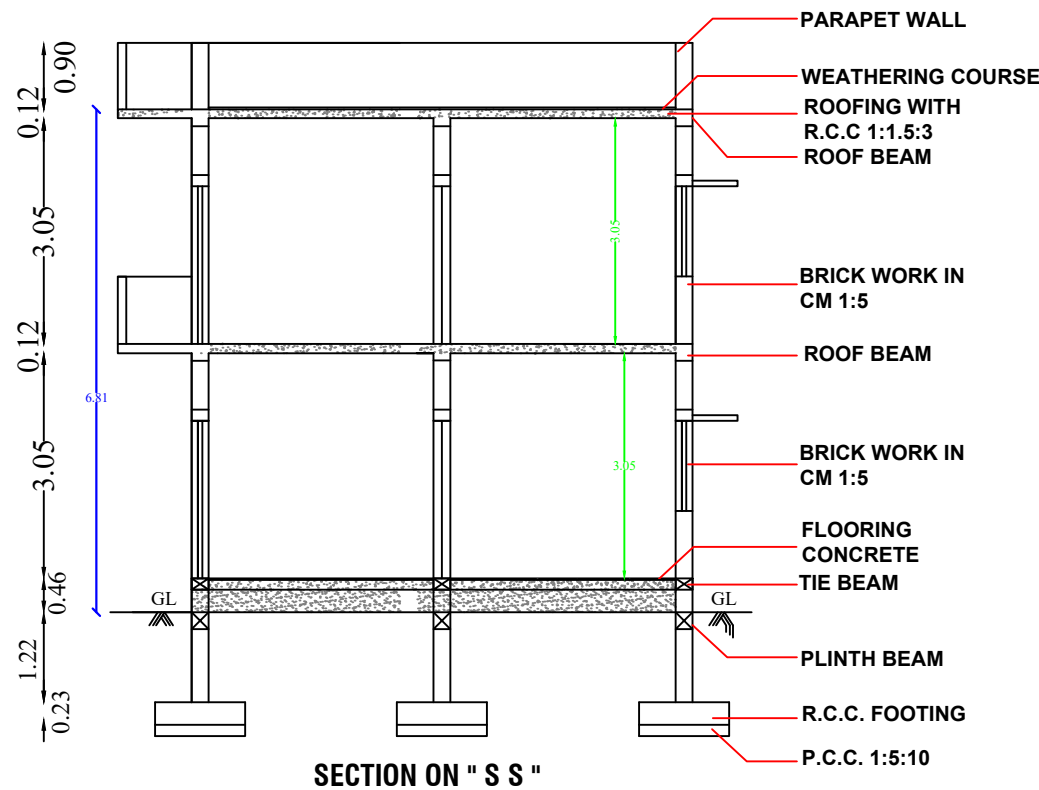
SECTION ON " S S "
