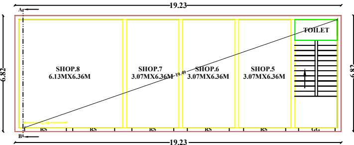
GROUND FLOOR [PART-I] COMMERCIAL - PLAN
