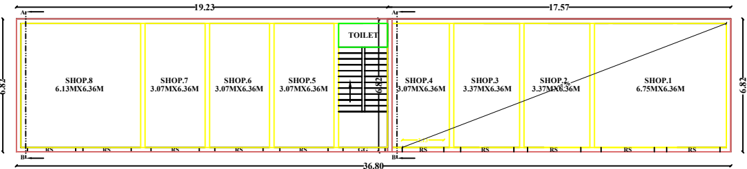
EXISTING APPROVED GROUND FLOOR [PART-I] COMMERCIAL - PLAN
