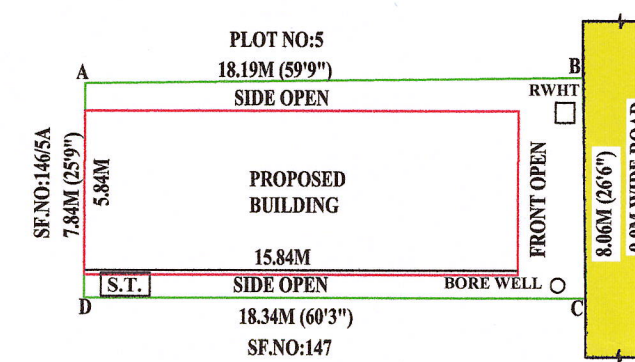
SITE PLAN
