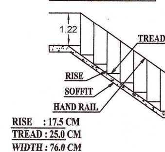
STAIRCASE DETAILS (NTS)
