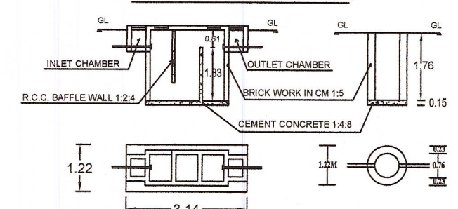
DETAILS OF SEPTIC TANK & SOAK PIT.
