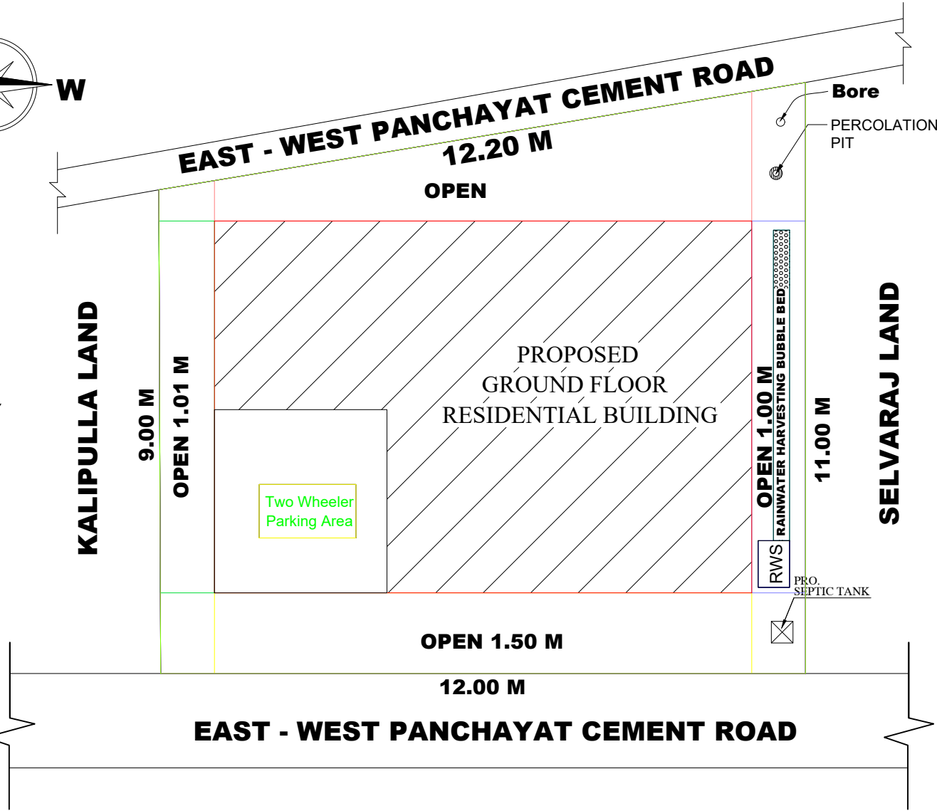
SITE PLAN (SCALE 1:1)
