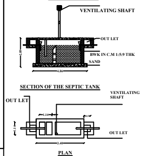
SEPTIC TANK
