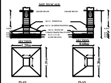
COLUMN FOOTING DETAILS
