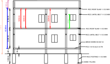
SECTION "AB"
