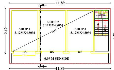
GROUND FLOOR - COMMERCIAL PLAN
