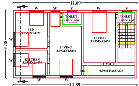
GROUND FLOOR - RESIDENTIAL PLAN
