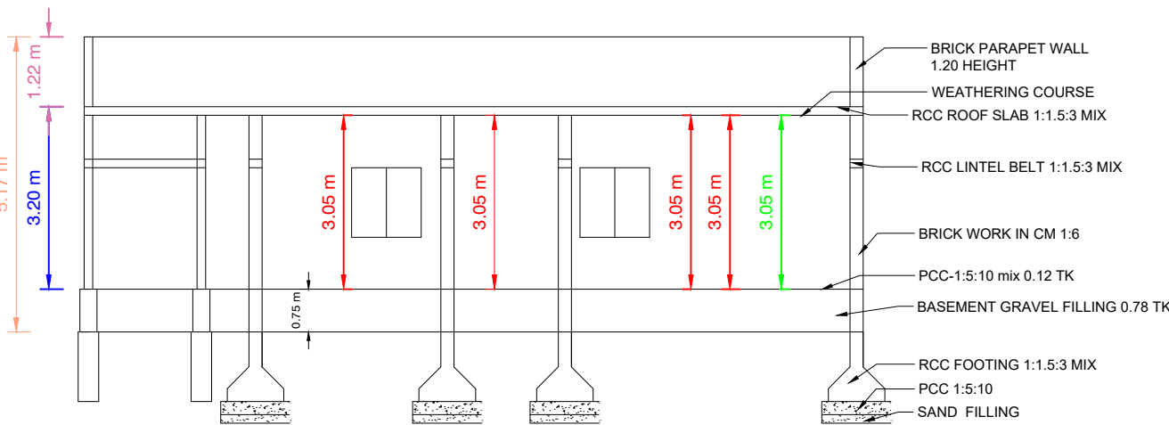
SECTION"AB"
