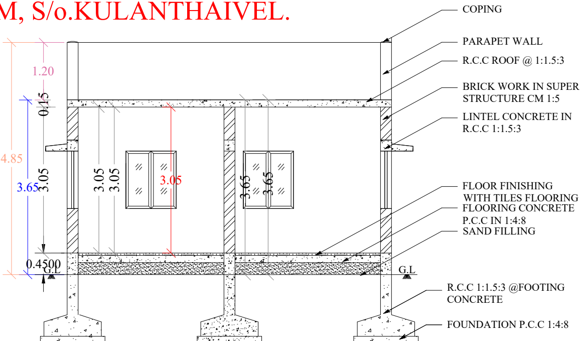
SECTION-AB
