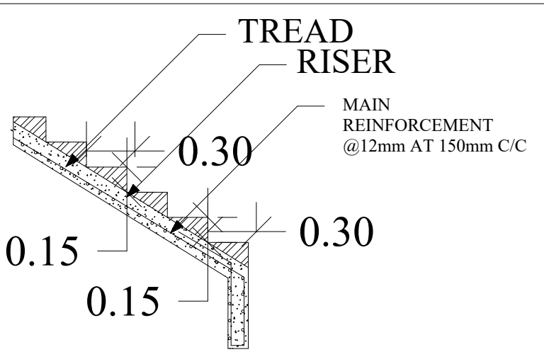
STAIRCASE DETAILS
