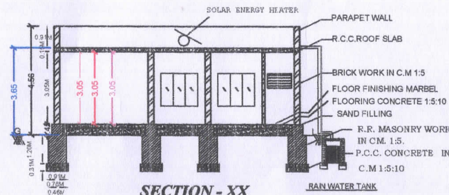
SECTION - XX
