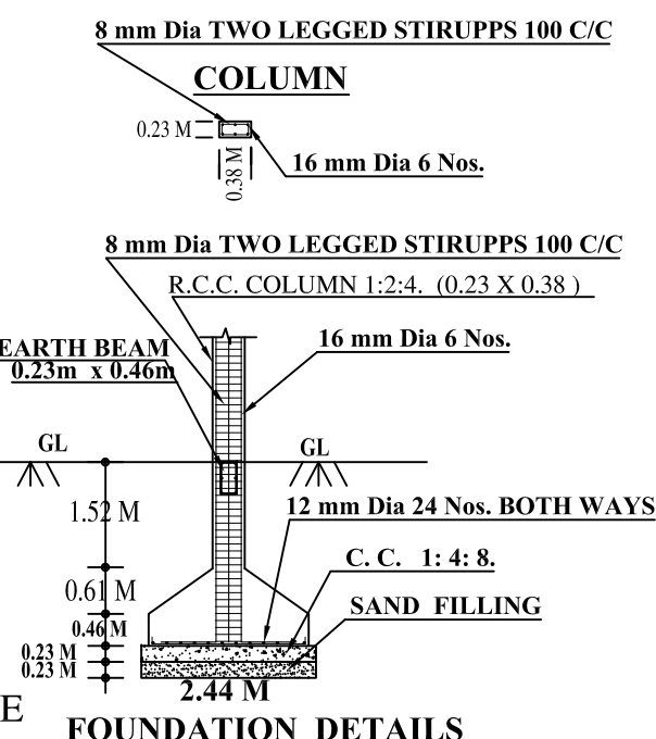
FOUNDATION DETAILS
