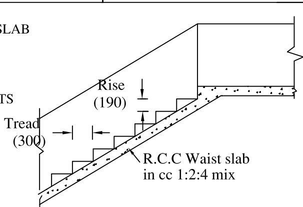
STAIRCASE DETAILS
