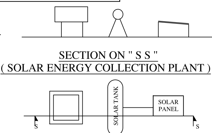
PLAN ( SOLAR ENERGY COLLECTION PLANT )
