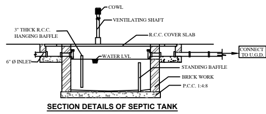
SECTION DETAILS OF SEPTIC TANK
