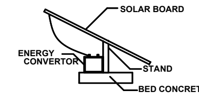
LONGITUDINAL SECTION FOUNDATION DETAILS
