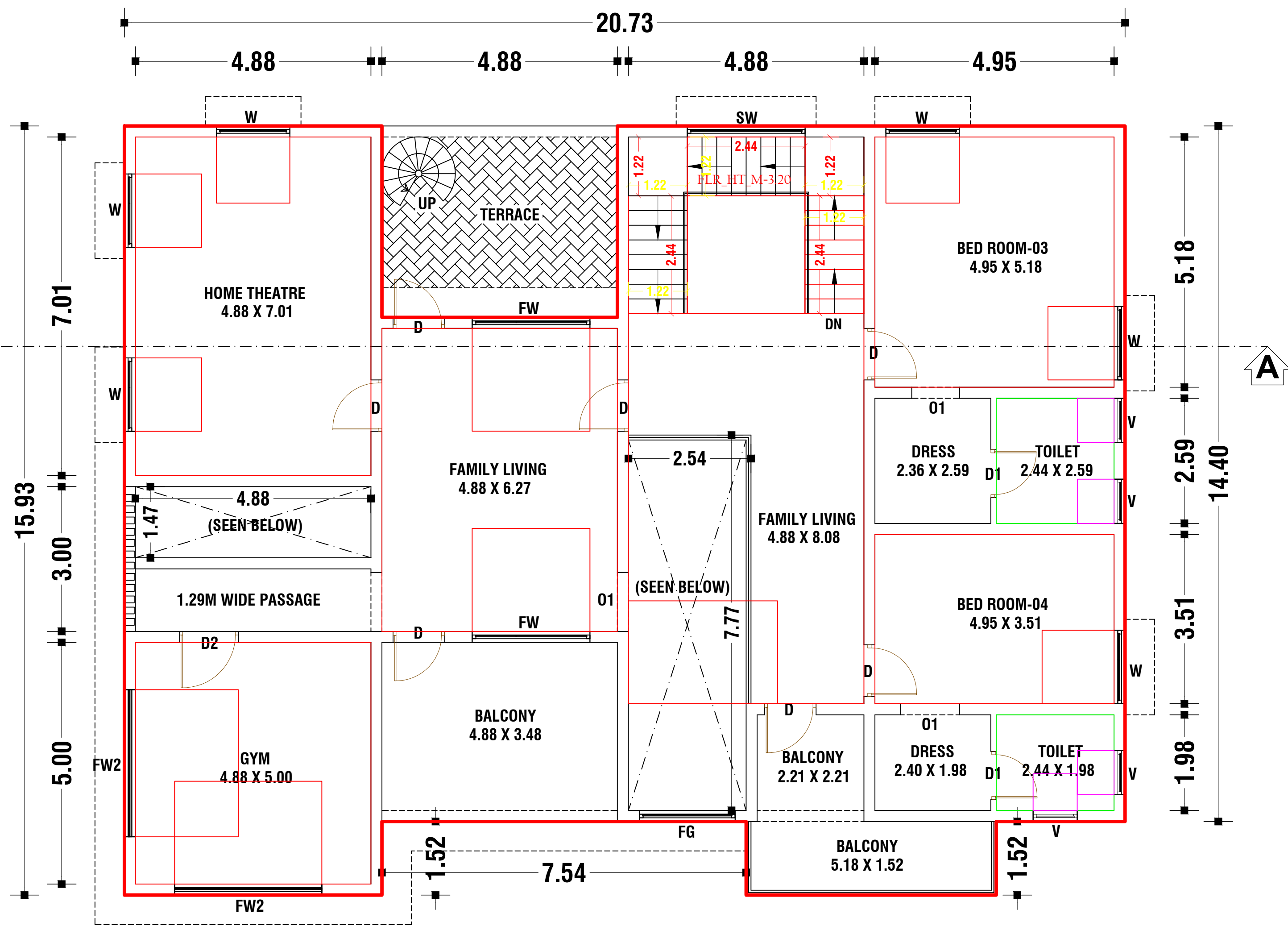
NORTH FACING FIRST FLOOR PLAN
