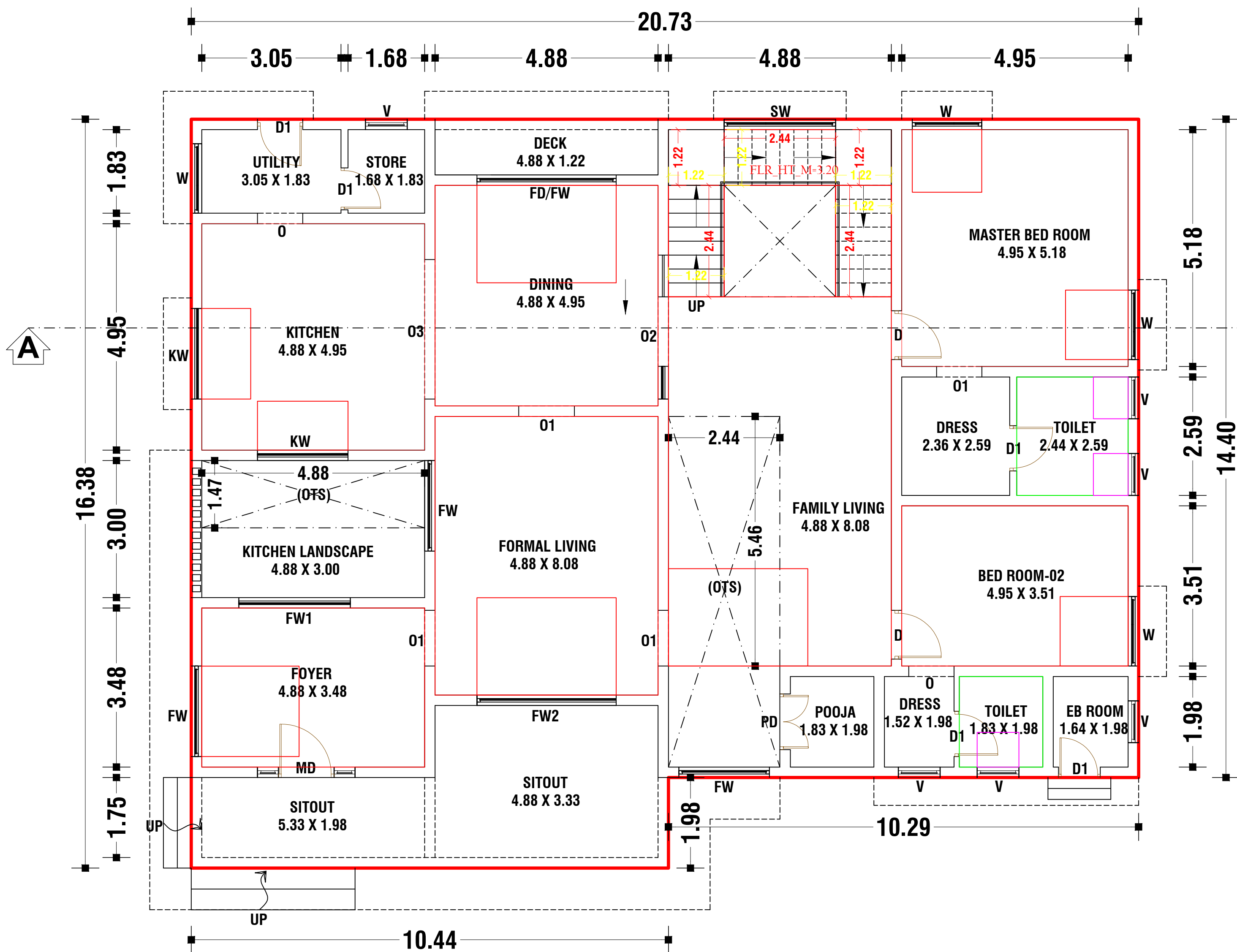
NORTH FACING GROUND FLOOR PLAN
