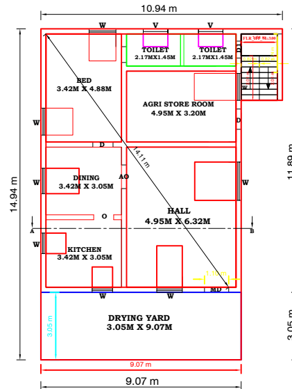
AGRI FARM HOUSE & DRYING YARD - PLAN
