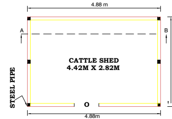
CATTLE SHED - PLAN
