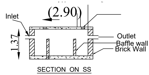
RAIN WATER HARVESTING TANK
