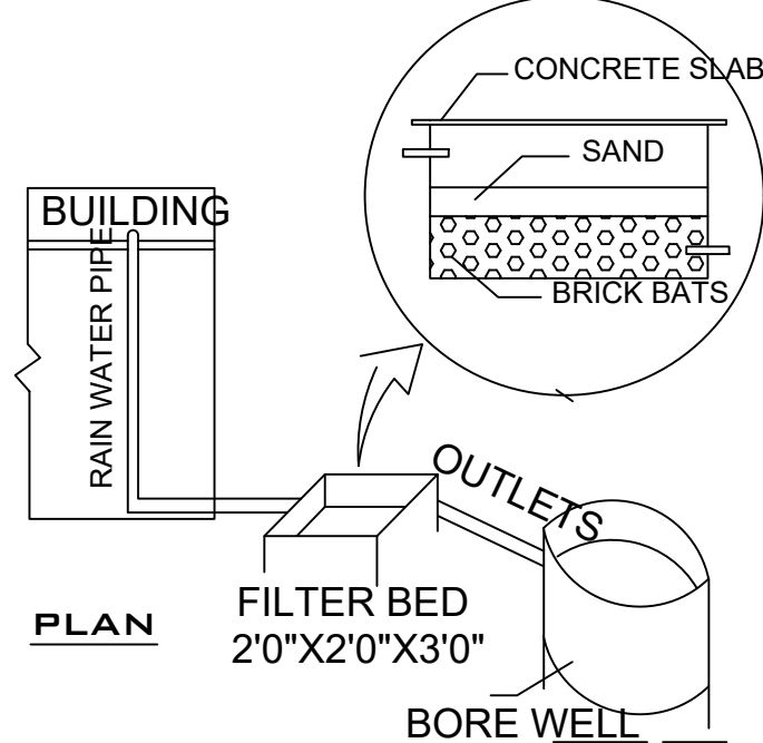
RAIN WATER HARVESTING TANK
