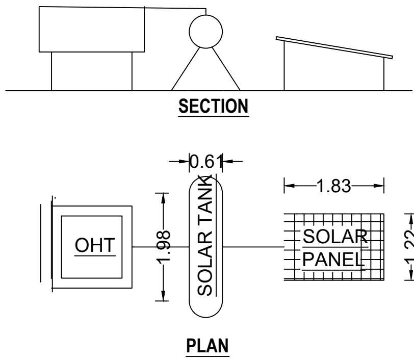
SOLAR SYSTEM
