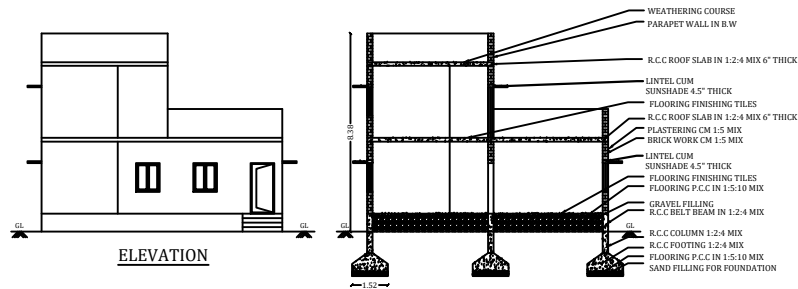
SECTION AB
