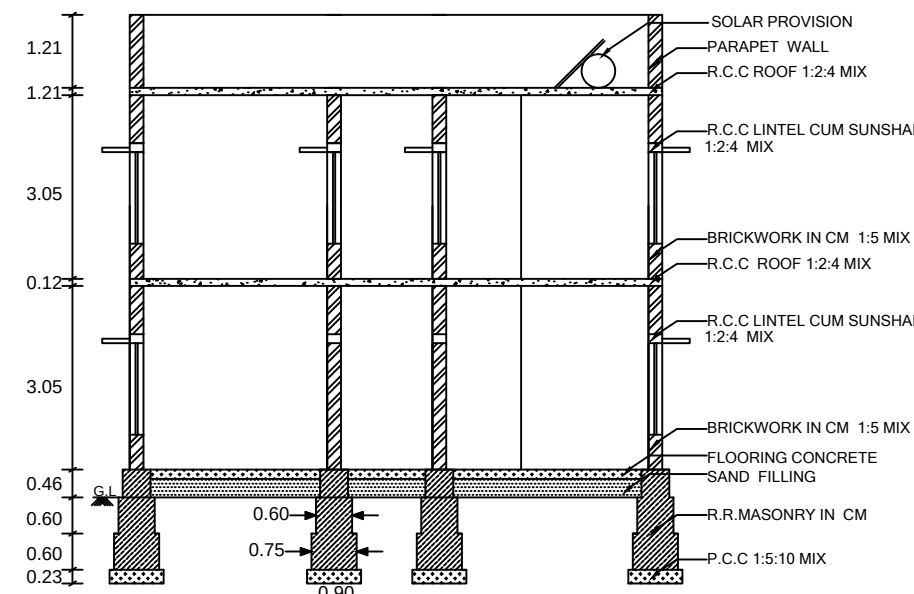
SECTION ON 'ABC'
